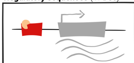
Regulatory sequences (TFBSs)
